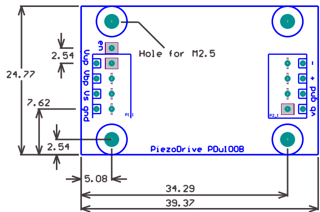
Figure 11. Top View (mm)
