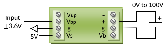
100 V Piezo stack driver with bipolar input and 50 V bias
