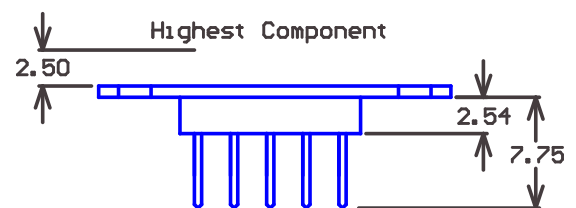
Figure 13. Left elevation: PDU100B-PCB (mm)
