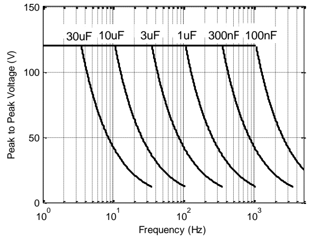
Figure 3. 60 V range power bandwidth
