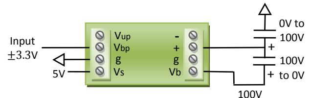
100 V Three-wire bender driver with bias
