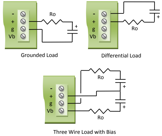
Figure 8. Noise reduction using output resistance
