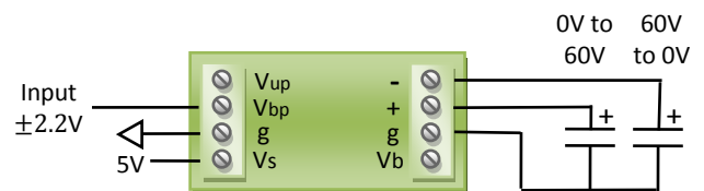
60 V Push-pull stack driver or bender driver
