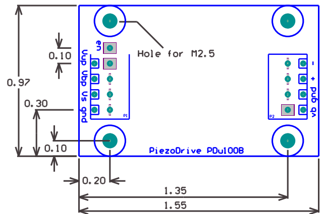
Figure 10. Top view (Inches)
