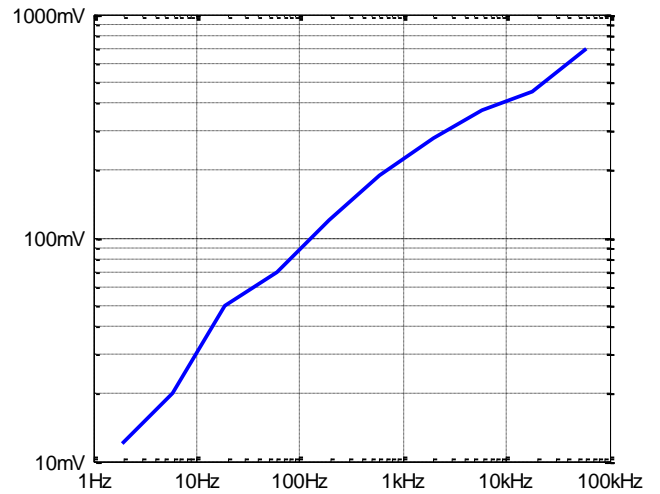
Figure 9. RMS output noise versus bandwidth
