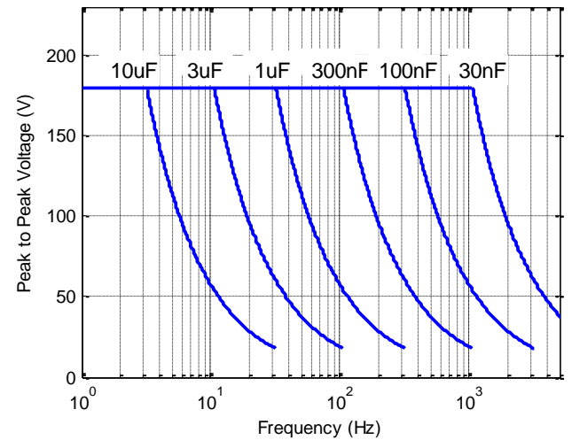
Figure 4. 90 V range power bandwidth
