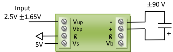
\pm 90 V Piezo bender driver with unipolar input
